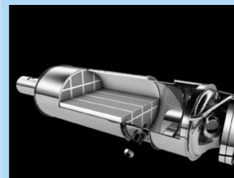
Diesel Particulate Filter (DPF).
